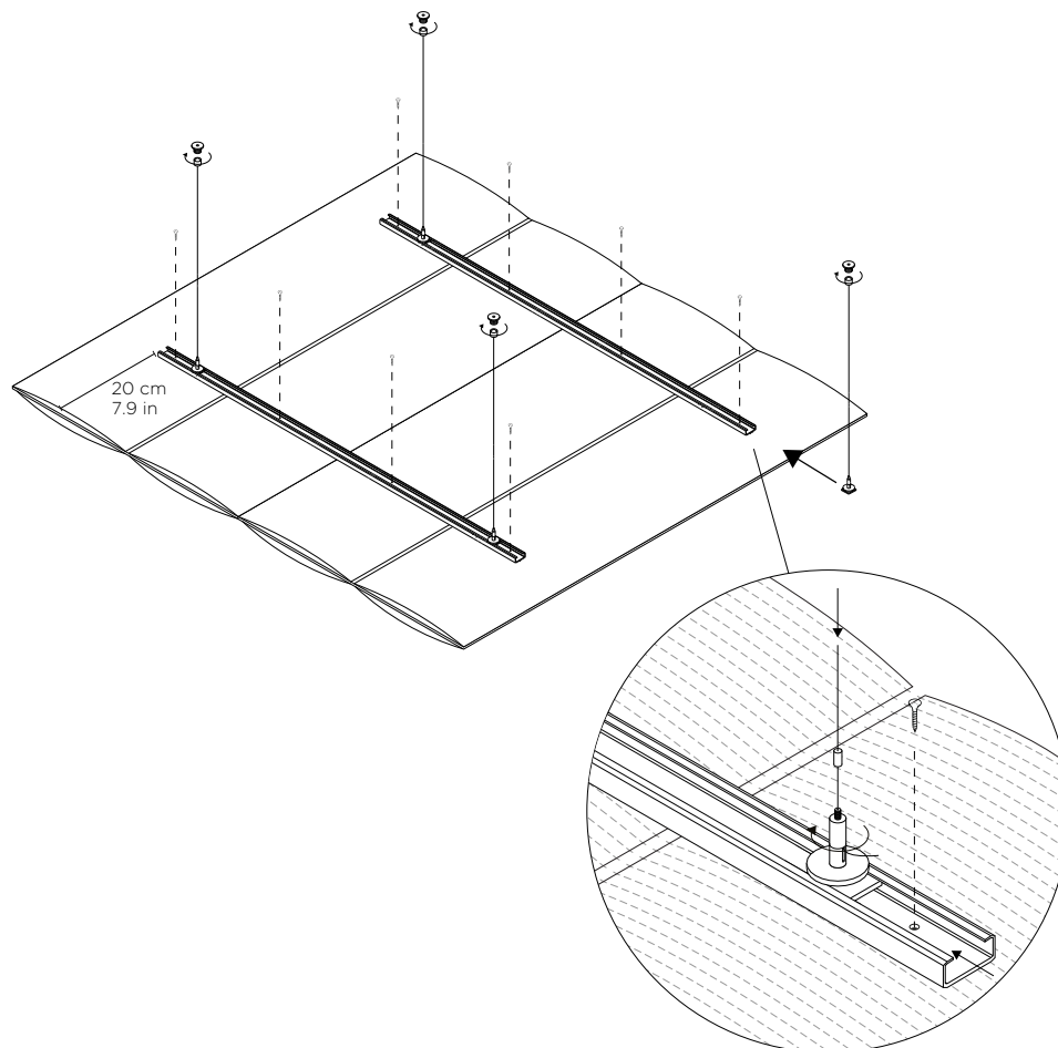
Axonomic view:
