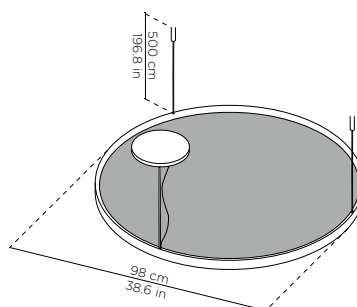
Axonometric view lateral cables:
